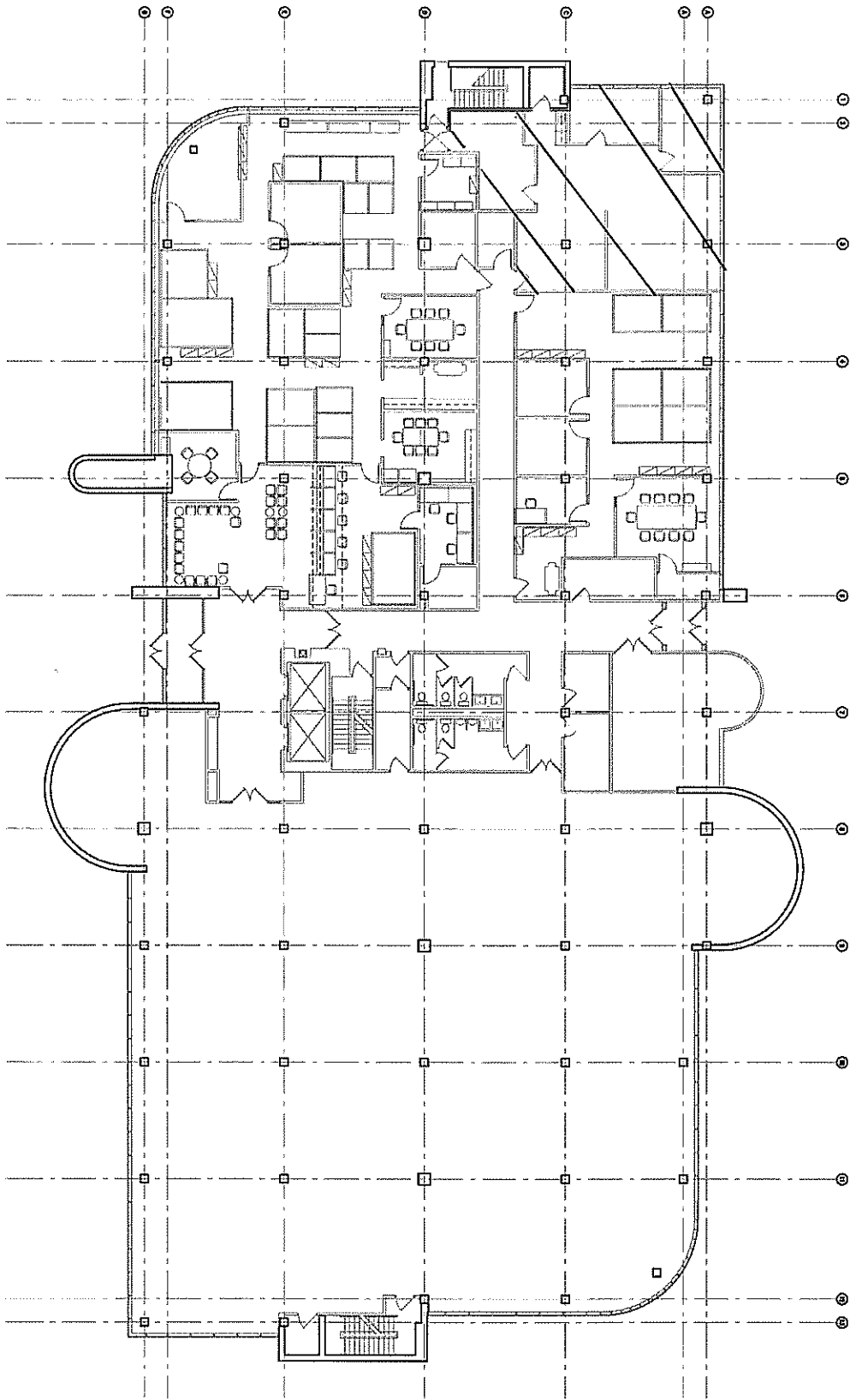
1 FIRST FLOOR EXISTING PLAN SCALE: 1/8" = 1'-0"
