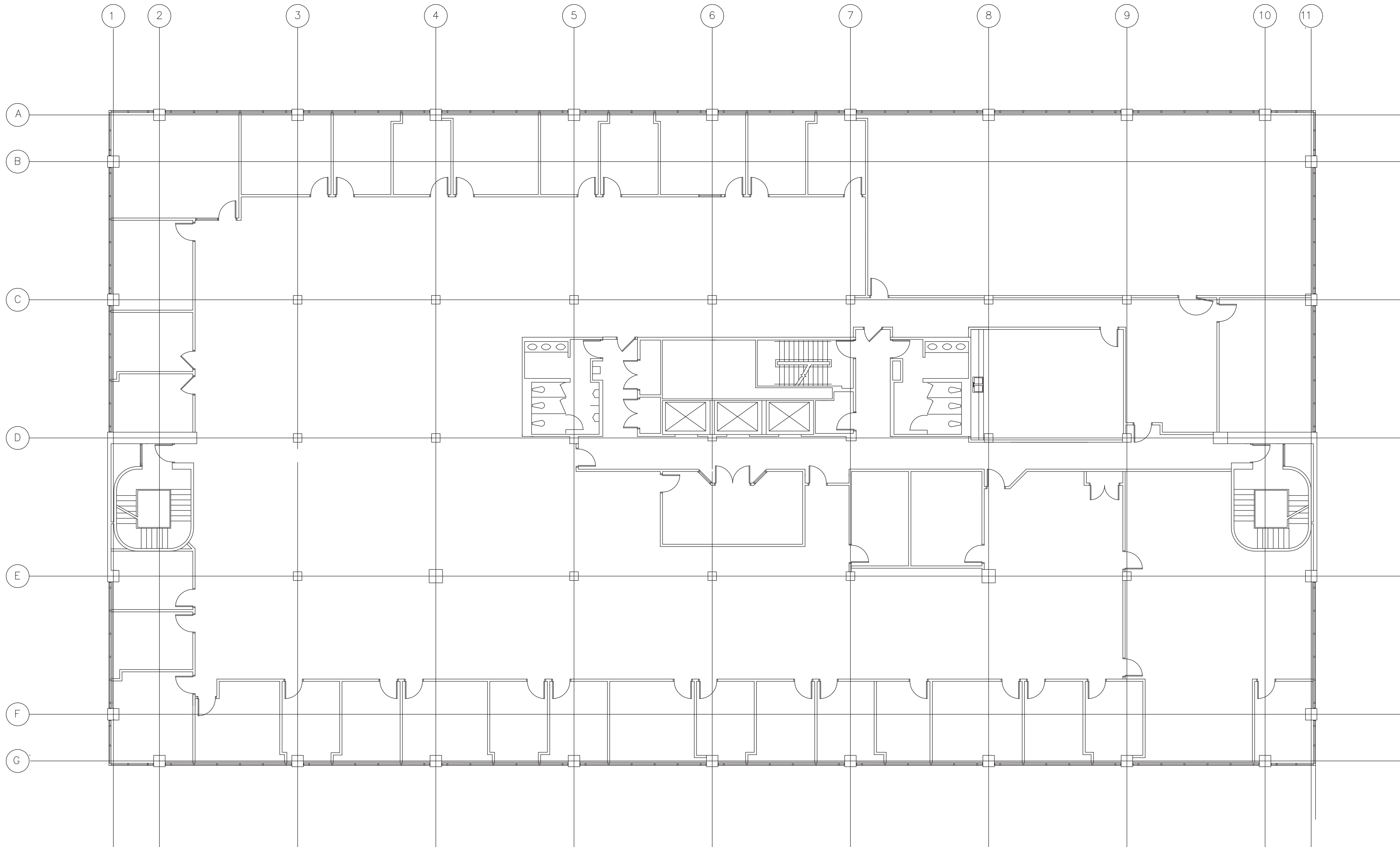
1 FOSTER PLAZA SIX, SIXTH FLOOR EXISTING CONDITIONS A1 SCALE: 1/8" = 1'-0"
